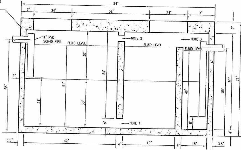
SIDE SECTION
